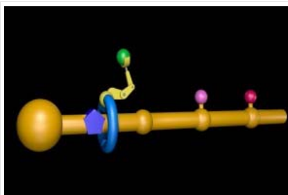
Molecule machine stacking molecules
